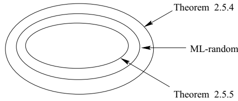
FIGURE 2.5. Three notions of ‘chaotic’ infinite sequences
