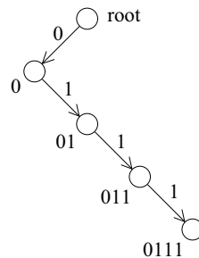
FIGURE 1.4. Binary tree for E(1) = 0 , E(2) = 01 , E(3) = 011 , E(4) = 0111
