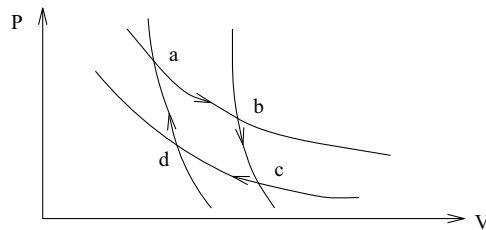
FIGURE 8.10. Carnot cycle
