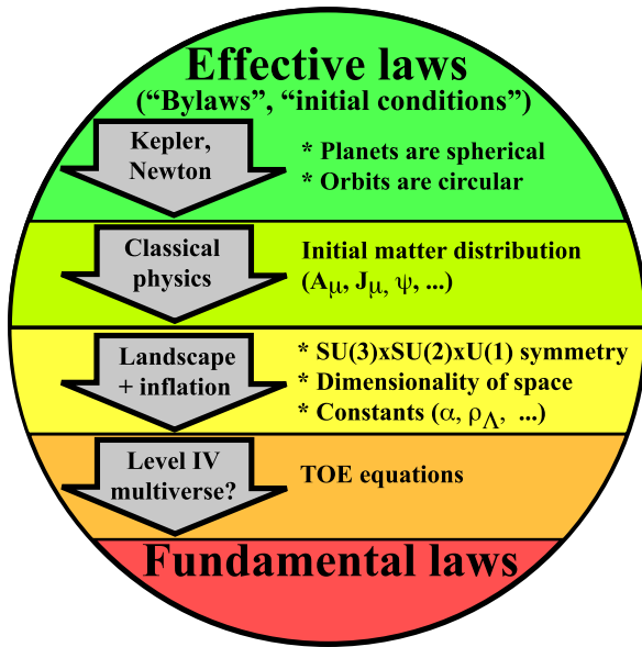
Fig. 2 The shifting boundary ( horizontal lines ) between fundamental laws and environmental laws/initial conditions. Whereas Ptolemy and others had argued that the circularity of planetary orbits was a fundamental law of nature, Kepler and Newton reclassified this as an initial condition, showing that the fundamental laws also allowed highly non-circular orbits. Classical physics removed from the fundamental law category also the initial conditions for the electromagnetic field and all other forms of matter and energy (responsible for almost all the complexity we observe), leaving the fundamental laws quite simple. A TOE with a landscape and inflation reclassifies many of the remaining “laws” as initial conditions, since they can differ from one post-inflationary region to another, but since inflation generically makes each such region infinite, it can fool us into misinterpreting these environmental properties as fundamental laws. Finally, if the MUH is correct and the Level IV multiverse of all mathematical structures (see Sect. 5) exists, then even the “theory of everything” equations that physicists are seeking are merely local bylaws in Rees’ terminology [41], differing across the ensemble
