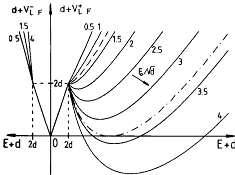
Fig. 11.24. The effective potential (11.179) as a function of E+d for various external forces F_0/\sqrt{d} and for the cosine potential f(x) = -d \cos x . The effective potential V_{LF}^+(V_{LF}^-) for positive (negative) velocities is plotted to the right (left). The effective potential for the critical force F_{01}/\sqrt{d} = 4/\pi is shown by a broken line and for the critical force F_{02}/\sqrt{d} = 3.3576 by a broken line with dots
