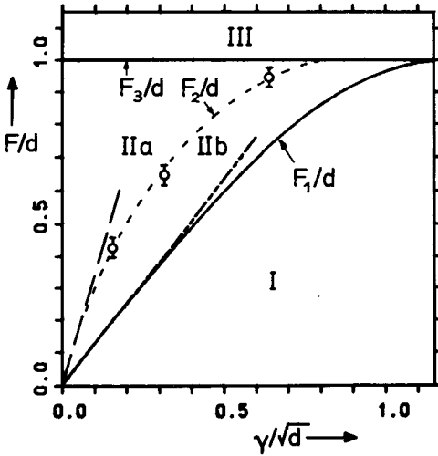
Fig. 11.26. The three critical forces F_1/d , F_2/d and F_3/d as a function of the friction constant \gamma/\sqrt{d} for the cosine potential (11.103). The straight lines --- and - - - are the low-friction approximations F_1 = (4/\pi)\sqrt{d}\gamma and F_2 = F_{02}\gamma , with F_{02} given by (11.196). The circles indicate extrapolations for \Theta \rightarrow 0 of the critical force F_2/d calculated with the matrix continued-fraction method. For the meaning of Regions I, IIa, IIb and III, see text
