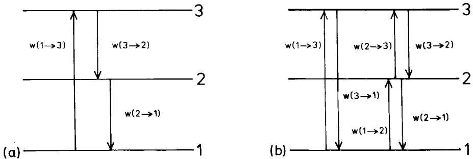
Fig. 6.1. Detailed balance is violated in (a). The probability current is given by S = w(1 \rightarrow 3)W_1 = w(3 \rightarrow 2)W_3 = w(2 \rightarrow 1)W_2 . If w(i \rightarrow j) = w(j \rightarrow i)W_j/W_i detailed balance is fulfilled in (b)
