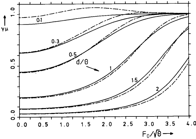
Fig. 11.19. The mobility times the damping constant according to the expansion (11.135) ( broken line ) compared with the exact result obtained by the matrix continued-fraction method of Sect. 11.5 ( full line ), as functions of the external force F_0/\sqrt{\Theta} = F/(\gamma|\sqrt{\Theta}) for different amplitudes d/\Theta of the cosine potential (11.103) and for \gamma/\sqrt{\Theta} = 0.05
