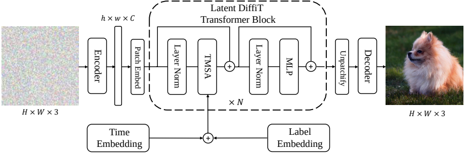
Fig. 3 – Overview of the latent DiffiT framework.
