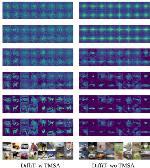
Fig. 2 – Side-by-side qualitative comparison of attention maps during the denoising process for models with and without TMSA. The denoising process starts from the top row.
